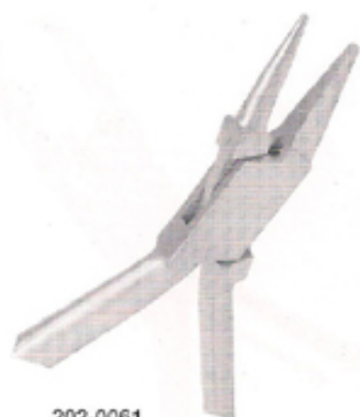
202-0061 Round & Flat Plier 5 1/2" (14 cm)
