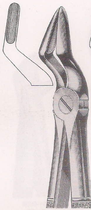
201-0032 Fig.52 Upper roots & canines with wider beak
